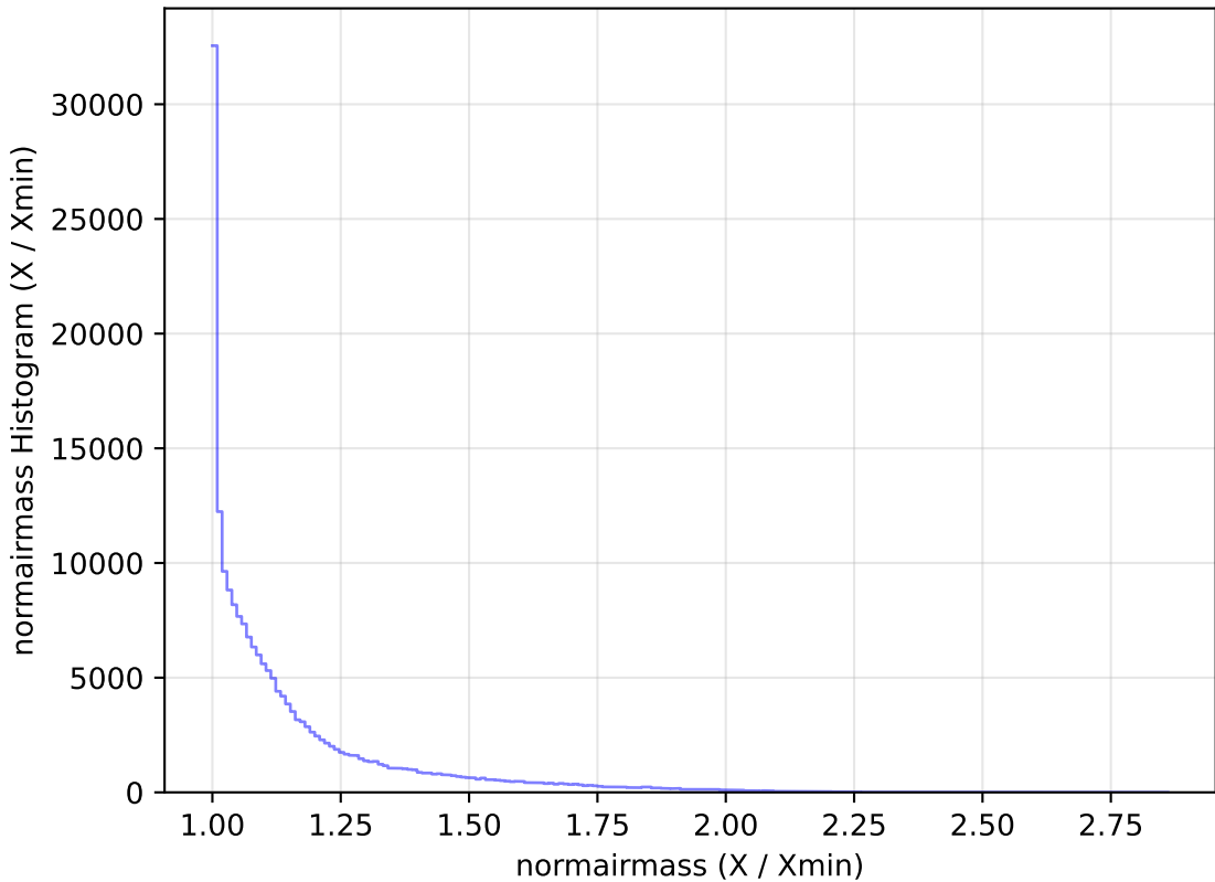
weather_cloudso12v3.4_10yrs All sky g band: normairmass Histogram
