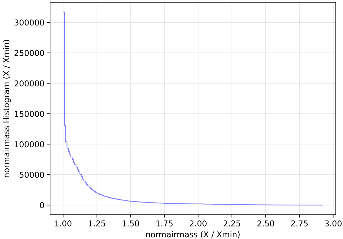
weather_cloudso12v3.4_10yrs All sky all bands: normairmass Histogram
