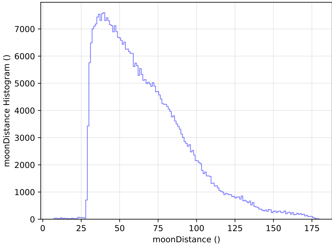
weather_cloudso12v3.4_10yrs WFD y band: moonDistance Histogram
