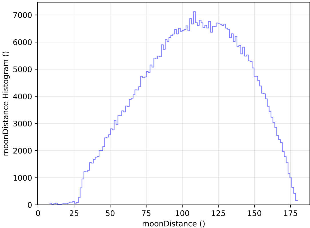
weather_cloudso12v3.4_10yrs WFD r band: moonDistance Histogram
