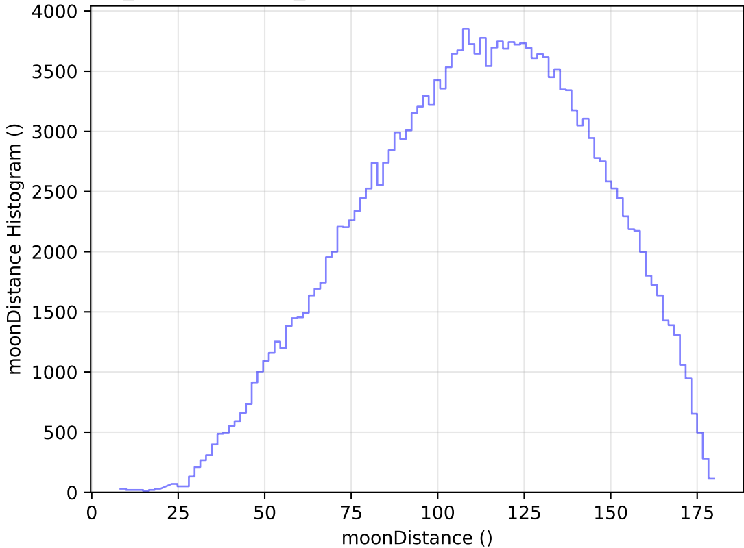
weather_cloudso12v3.4_10yrs WFD g band: moonDistance Histogram
