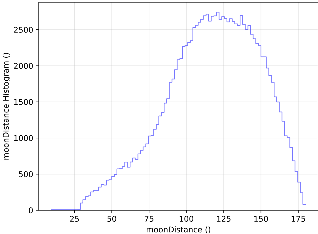
weather_cloudso12v3.4_10yrs All sky u band: moonDistance Histogram
