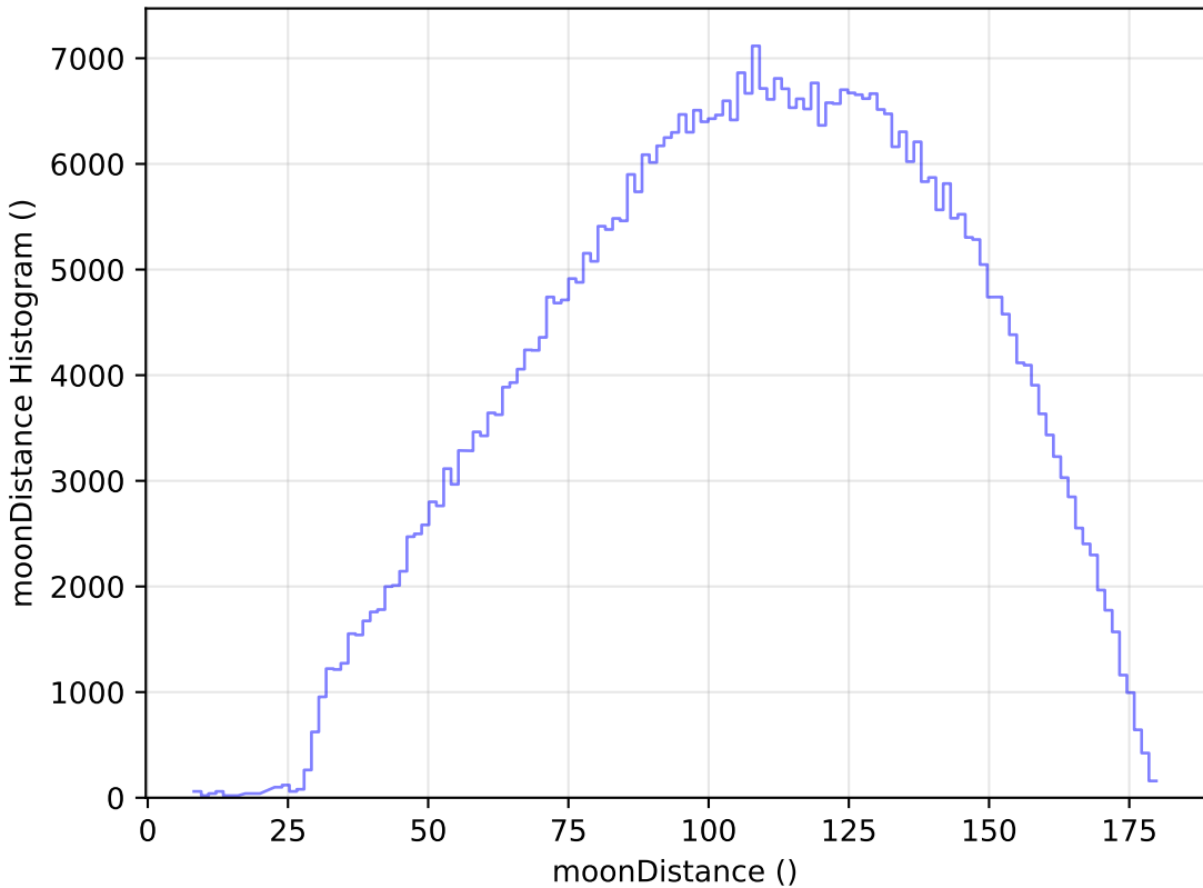
weather_cloudso12v3.4_10yrs All sky r band: moonDistance Histogram
