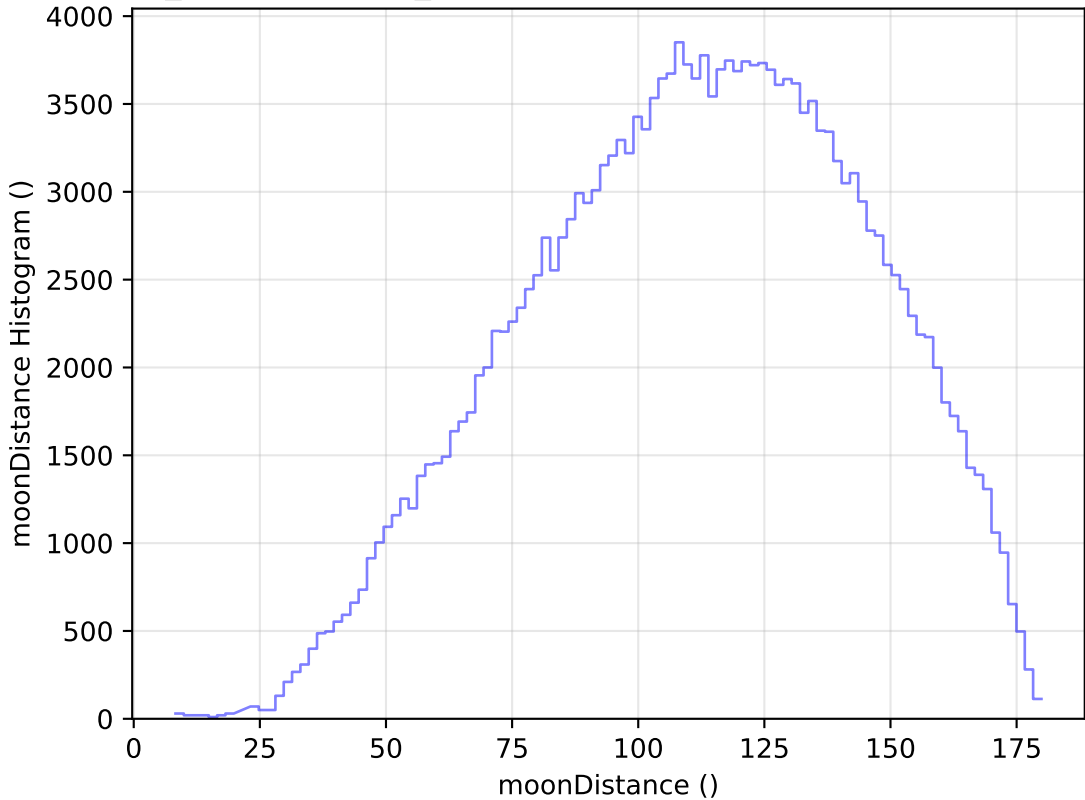
weather_cloudso12v3.4_10yrs All sky g band: moonDistance Histogram
