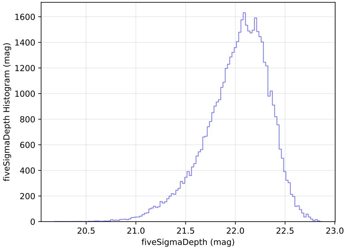
weather_cloudso12v3.4_10yrs Yr 1 y band: fiveSigmaDepth Histogram
