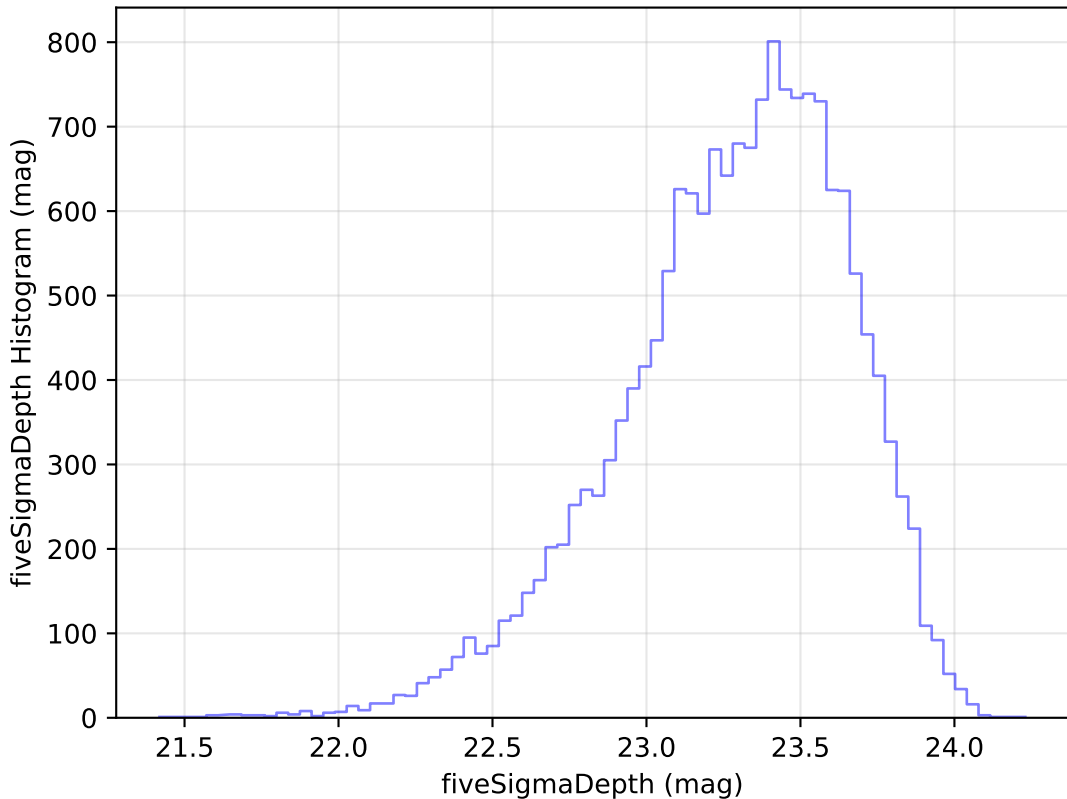
weather_cloudso12v3.4_10yrs Yr 1 u band: fiveSigmaDepth Histogram
