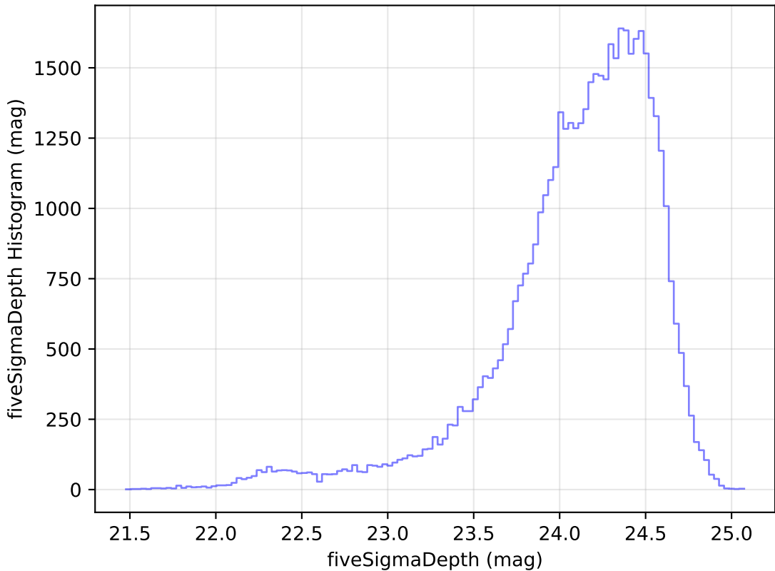
weather_cloudso12v3.4_10yrs Yr 1 r band: fiveSigmaDepth Histogram
