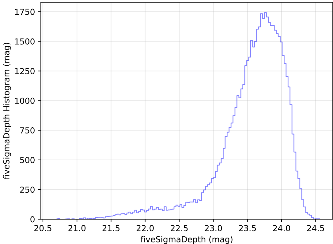
weather_cloudso12v3.4_10yrs Yr 1 i band: fiveSigmaDepth Histogram
