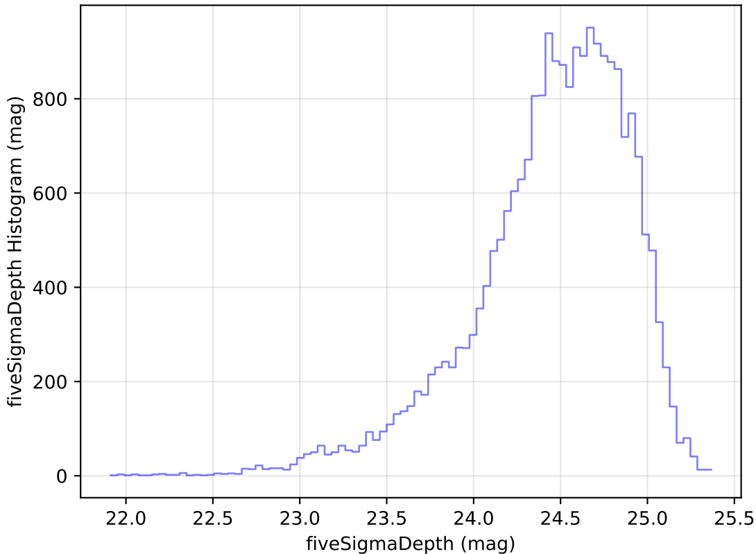
weather_cloudso12v3.4_10yrs Yr 1 g band: fiveSigmaDepth Histogram
