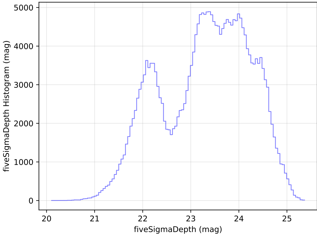
weather_cloudso12v3.4_10yrs Yr 1 all bands: fiveSigmaDepth Histogram
