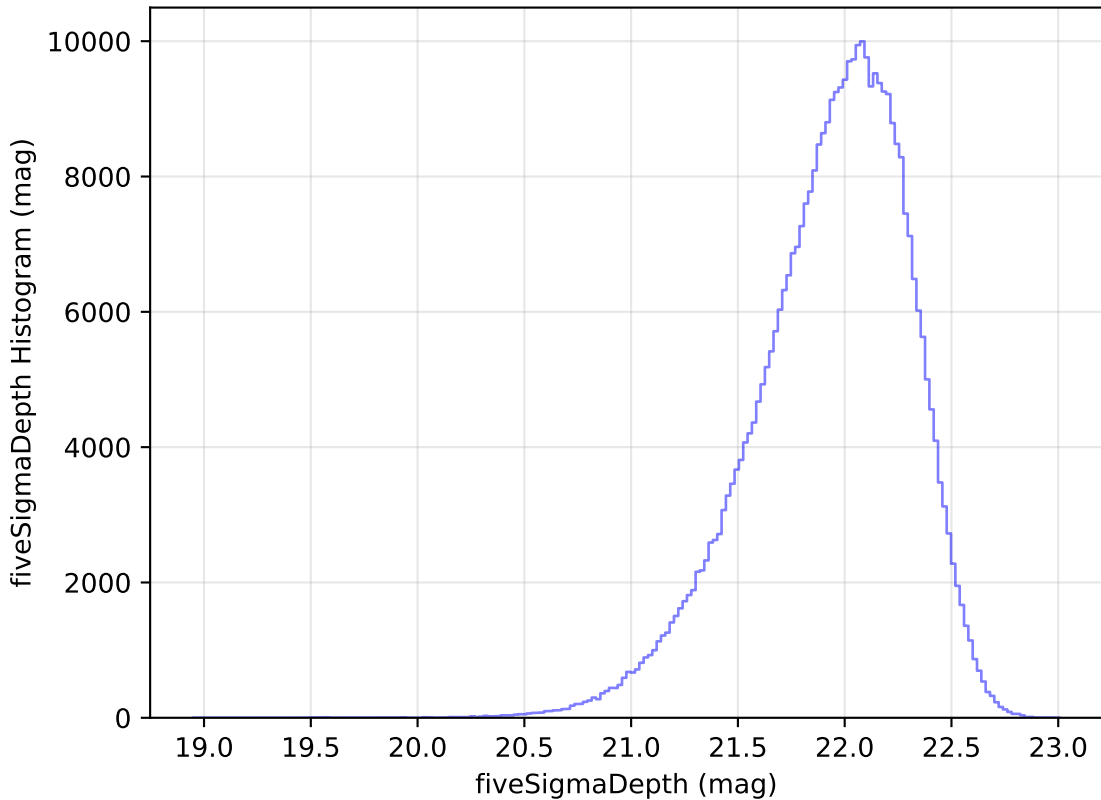
weather_cloudso12v3.4_10yrs WFD y band: fiveSigmaDepth Histogram
