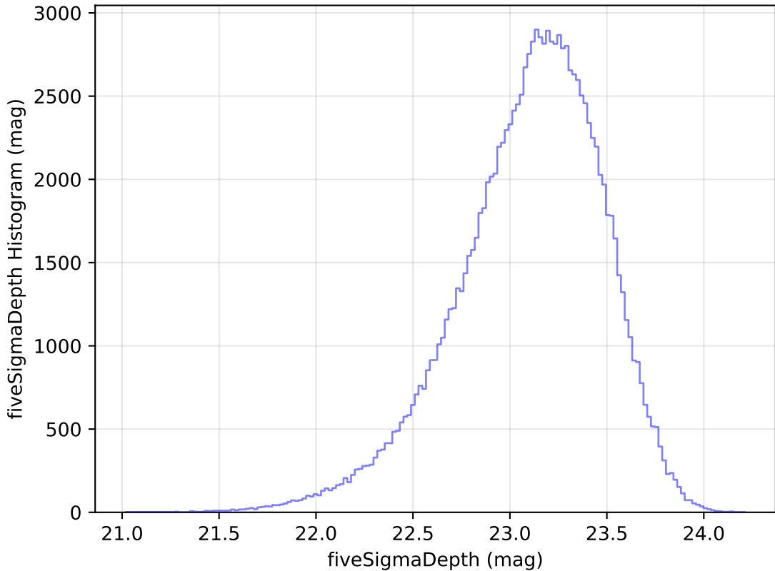
weather_cloudso12v3.4_10yrs WFD u band: fiveSigmaDepth Histogram
