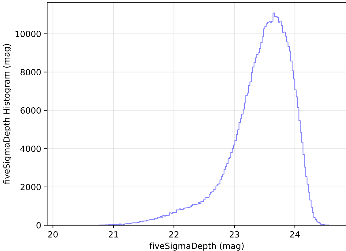
weather_cloudso12v3.4_10yrs WFD i band: fiveSigmaDepth Histogram
