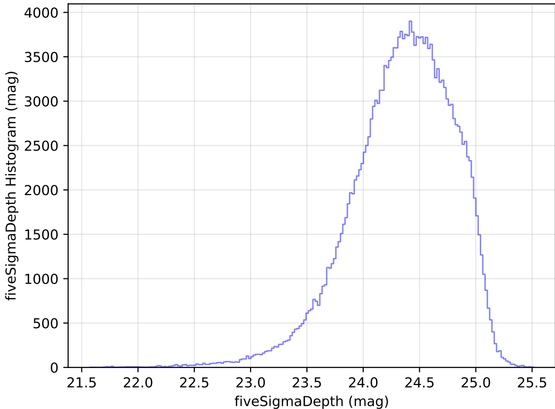
weather_cloudso12v3.4_10yrs WFD g band: fiveSigmaDepth Histogram
