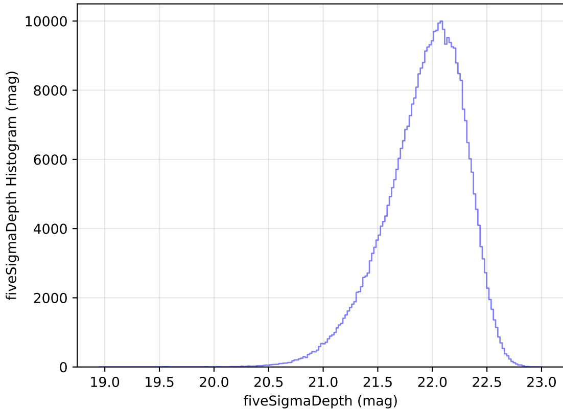
weather_cloudso12v3.4_10yrs All sky y band: fiveSigmaDepth Histogram
