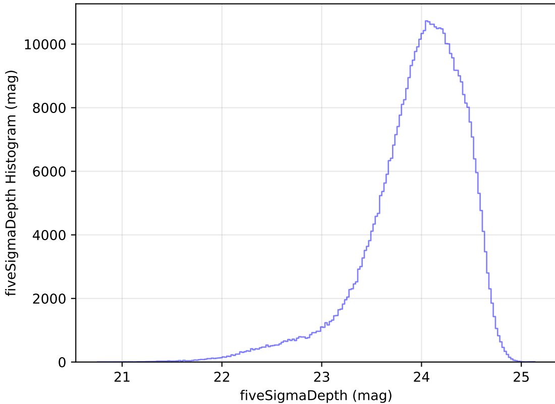
weather_cloudso12v3.4_10yrs All sky r band: fiveSigmaDepth Histogram
