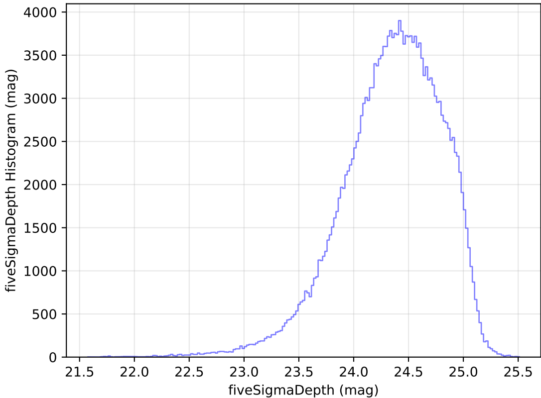
weather_cloudso12v3.4_10yrs All sky g band: fiveSigmaDepth Histogram
