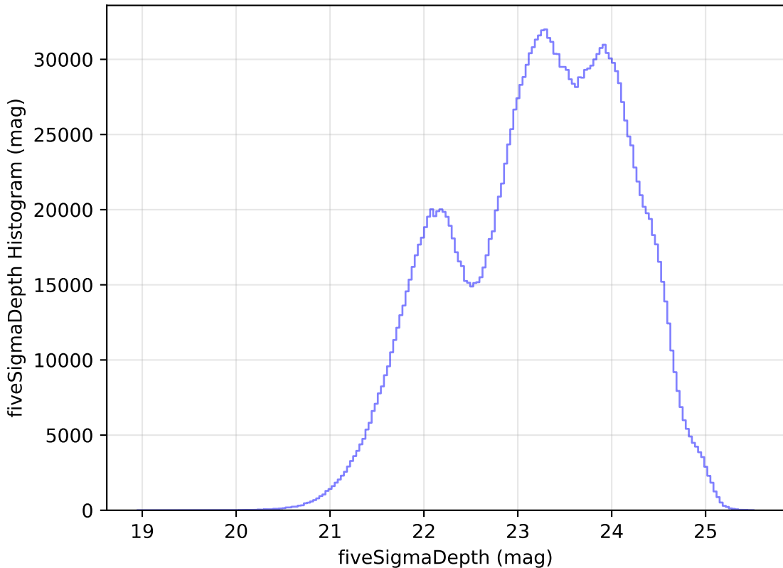
weather_cloudso12v3.4_10yrs All sky all bands: fiveSigmaDepth Histogram
