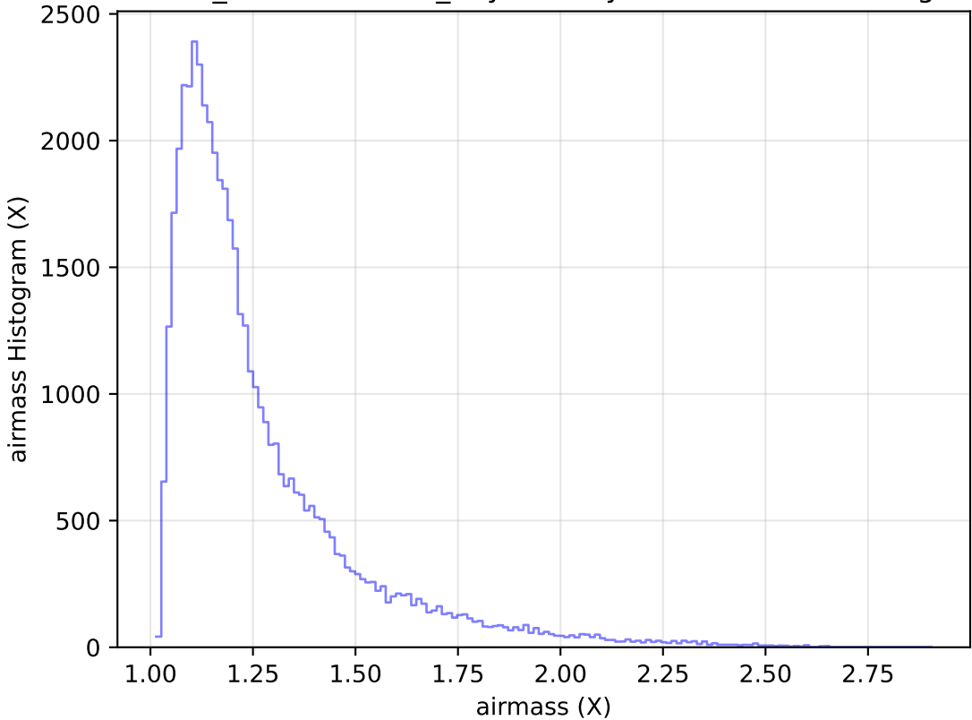
weather_cloudso12v3.4_10yrs Yr 1 y band: airmass Histogram
