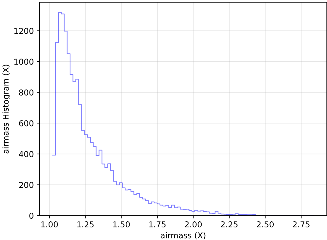
weather_cloudso12v3.4_10yrs Yr 1 u band: airmass Histogram
