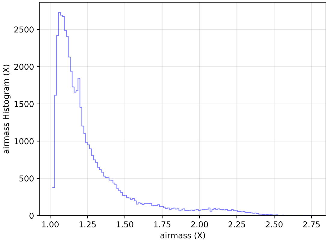
weather_cloudso12v3.4_10yrs Yr 1 r band: airmass Histogram
