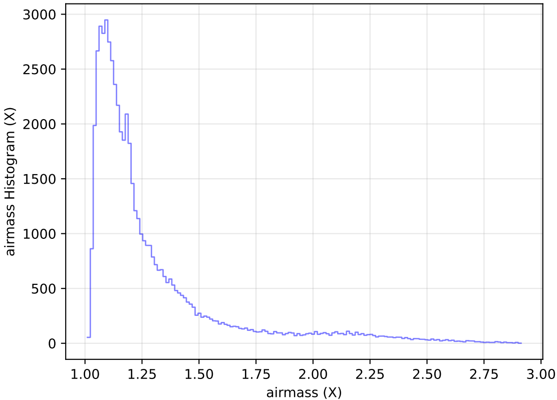
weather_cloudso12v3.4_10yrs Yr 1 i band: airmass Histogram
