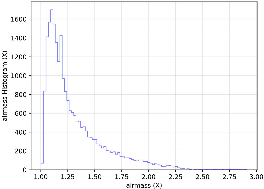
weather_cloudso12v3.4_10yrs Yr 1 g band: airmass Histogram
