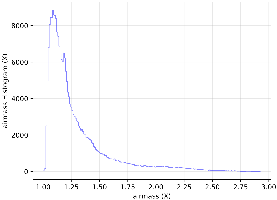
weather_cloudso12v3.4_10yrs Yr 1 all bands: airmass Histogram
