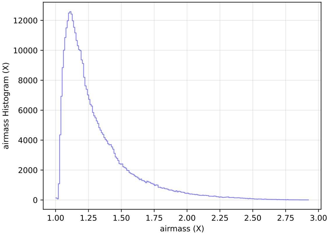
weather_cloudso12v3.4_10yrs WFD y band: airmass Histogram
