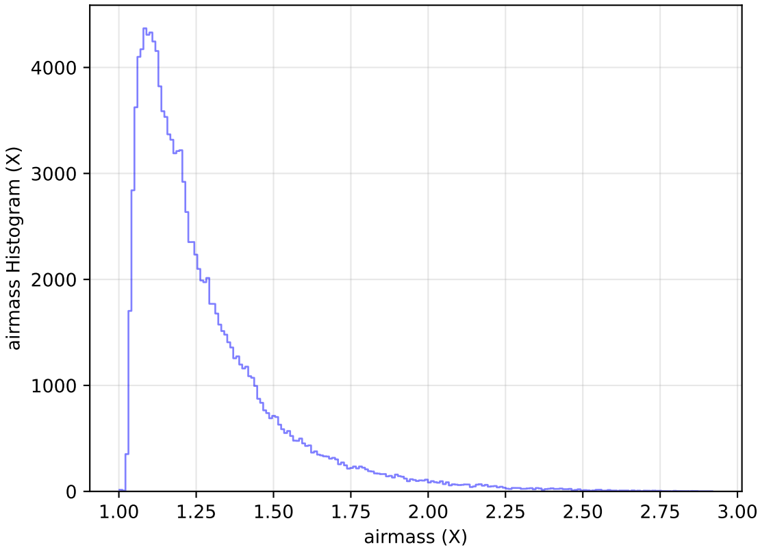
weather_cloudso12v3.4_10yrs WFD u band: airmass Histogram
