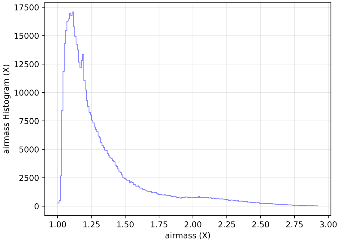
weather_cloudso12v3.4_10yrs WFD i band: airmass Histogram
