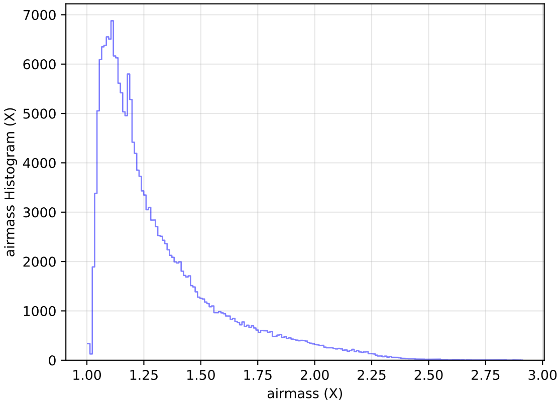
weather_cloudso12v3.4_10yrs WFD g band: airmass Histogram
