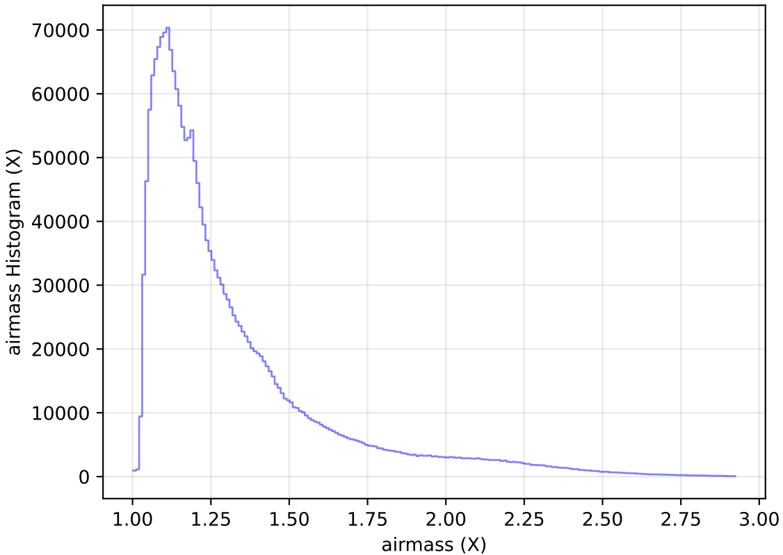
weather_cloudso12v3.4_10yrs WFD all bands: airmass Histogram
