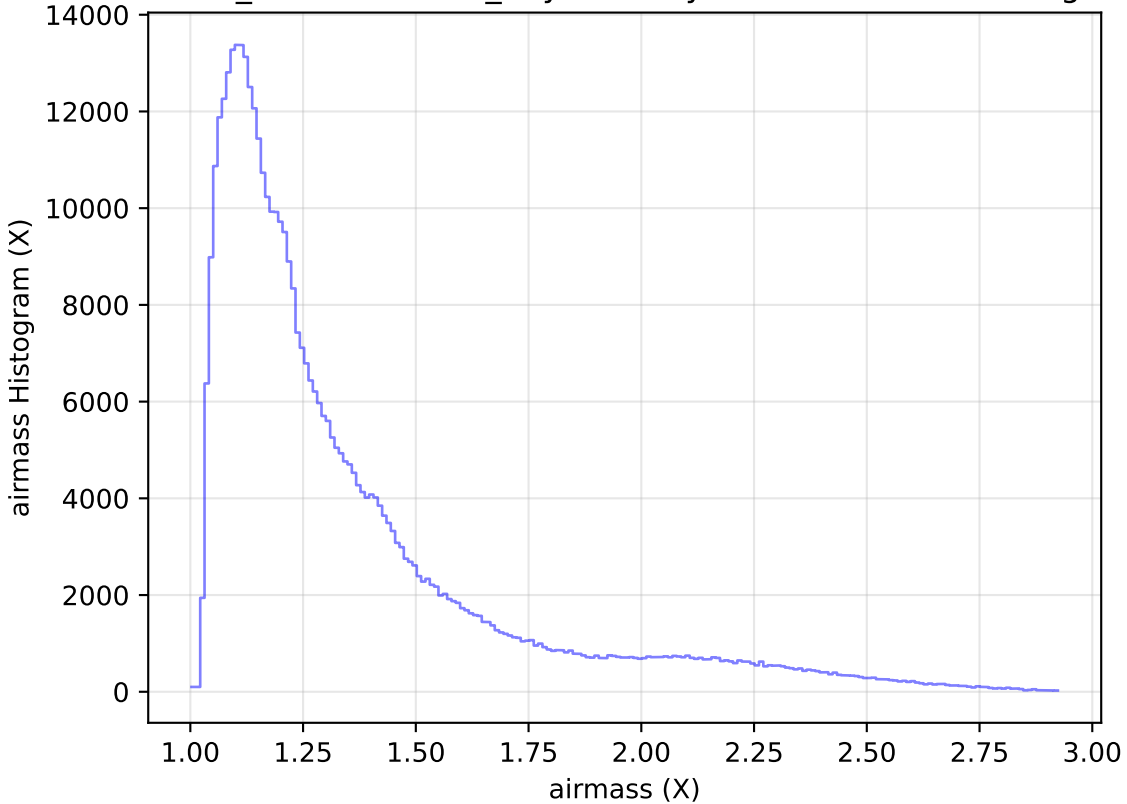
weather_cloudso12v3.4_10yrs All sky z band: airmass Histogram
