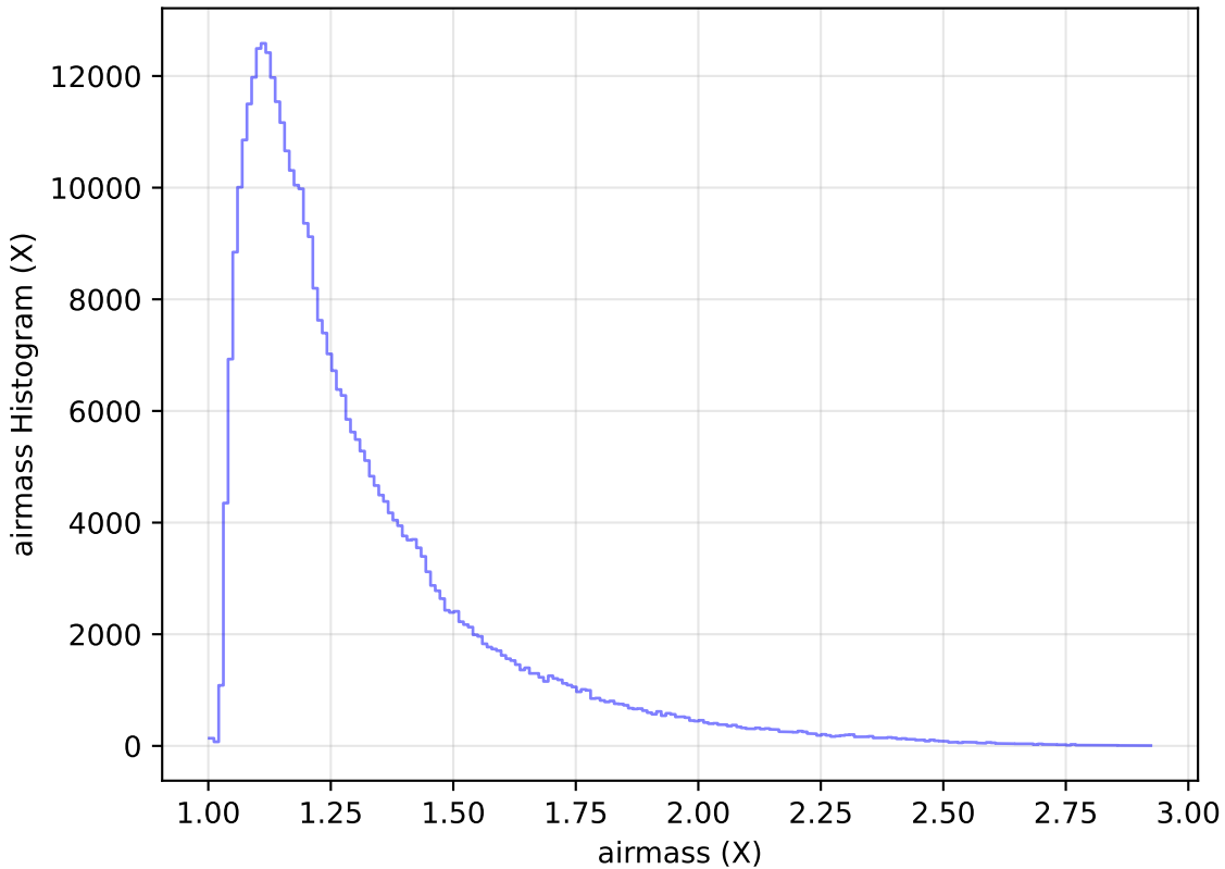
weather_cloudso12v3.4_10yrs All sky y band: airmass Histogram
