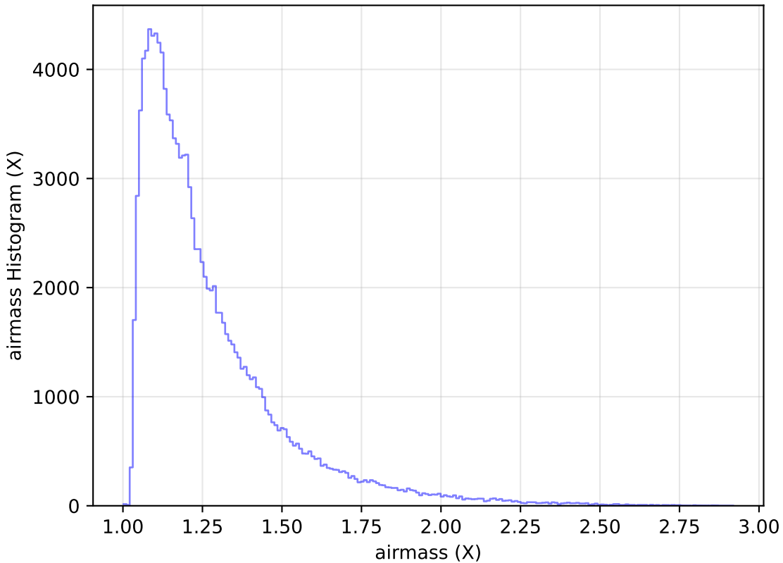
weather_cloudso12v3.4_10yrs All sky u band: airmass Histogram
