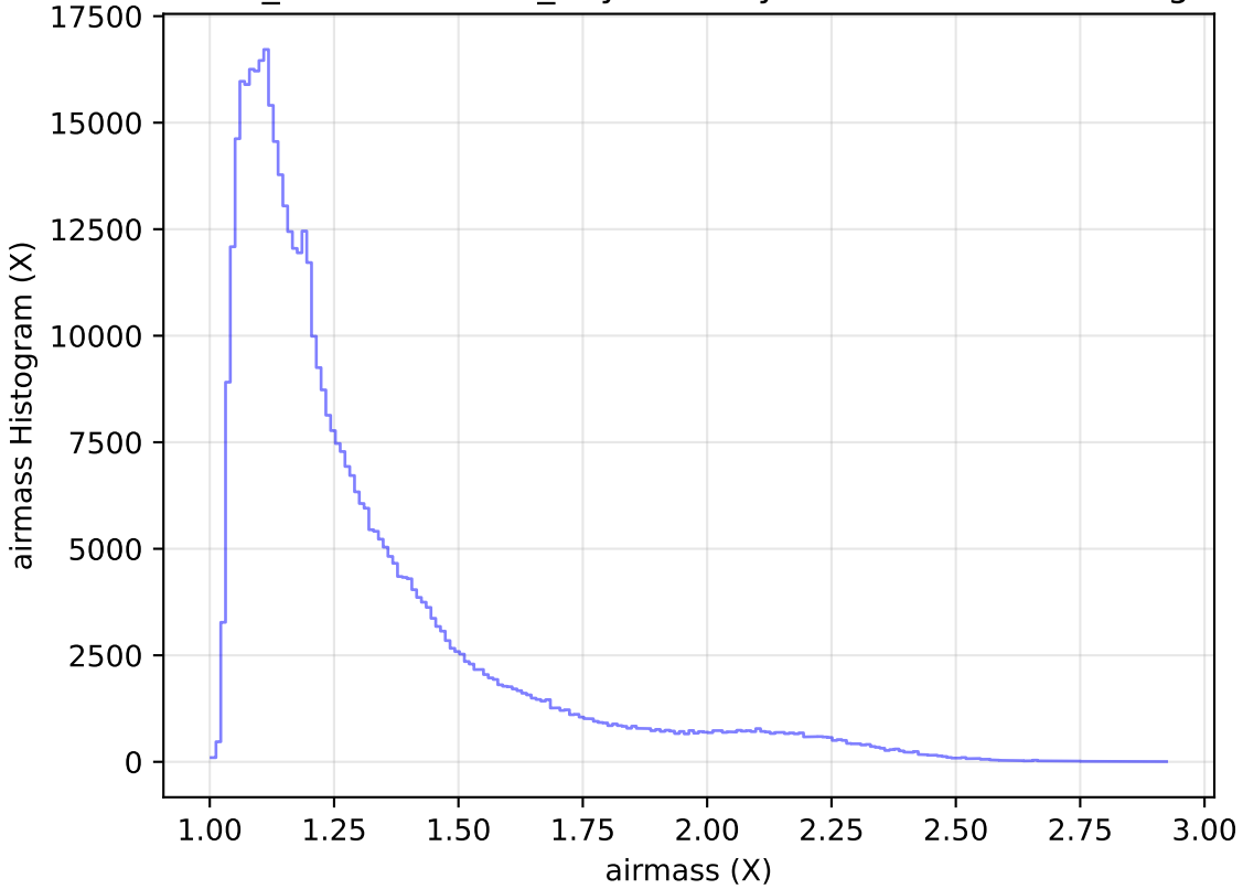
weather_cloudso12v3.4_10yrs All sky r band: airmass Histogram
