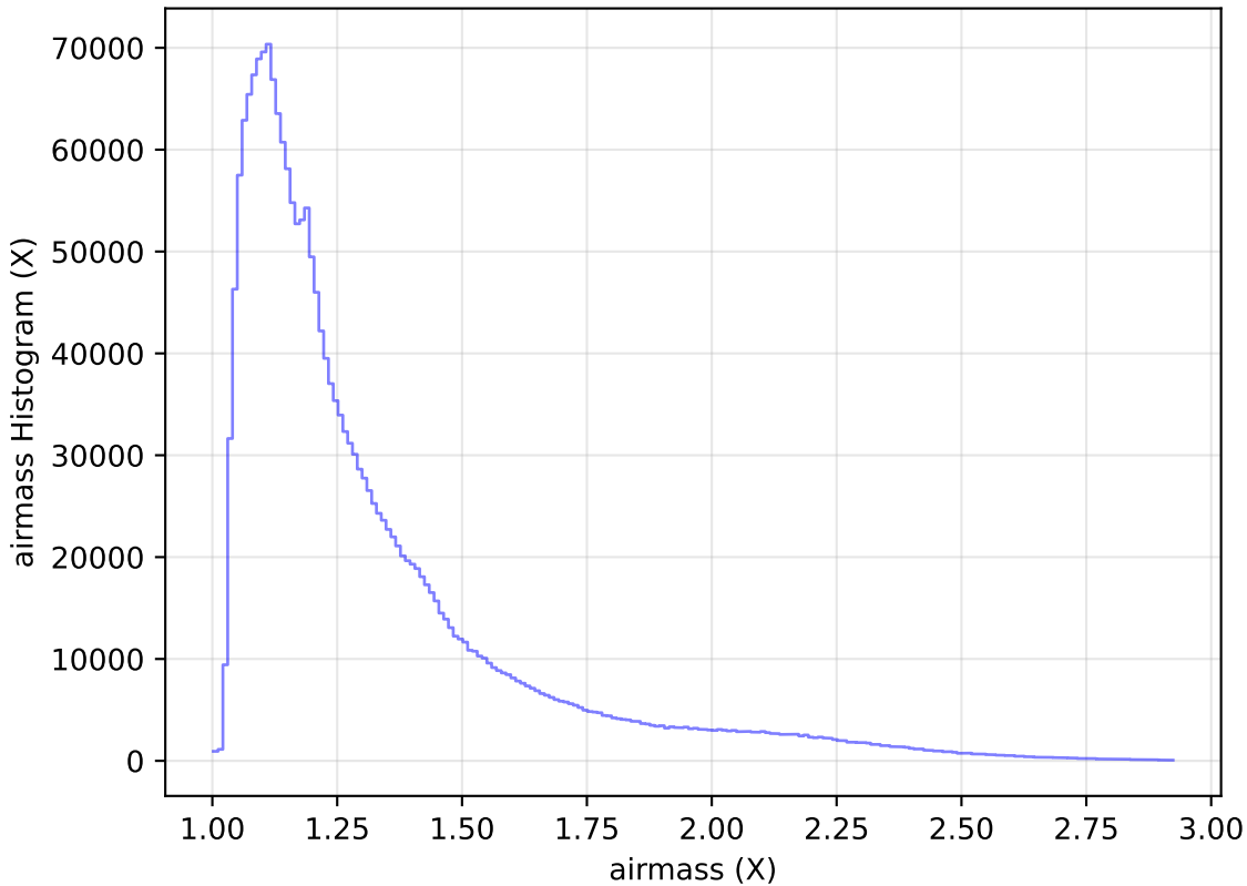
weather_cloudso12v3.4_10yrs All sky all bands: airmass Histogram
