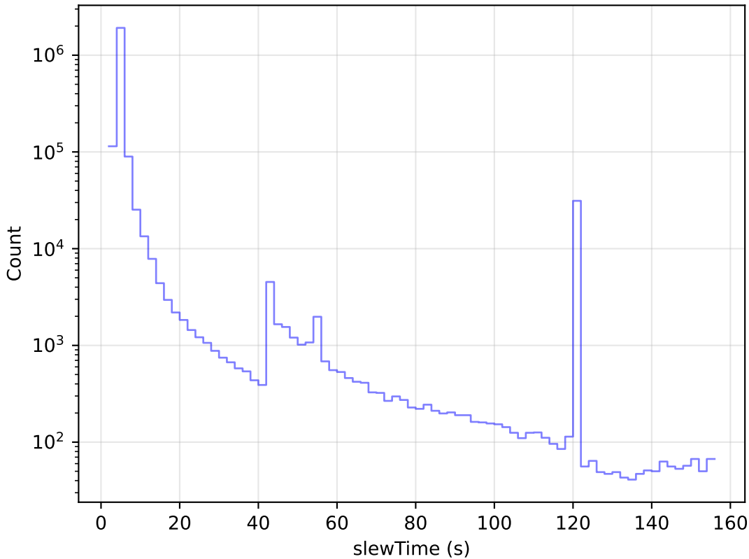
weather_cloudso12v3.4_10yrs All visits: Slew Time Histogram
