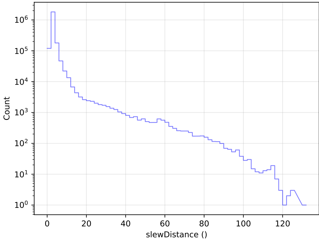
weather_cloudso12v3.4_10yrs All visits: Slew Distance Histogram
