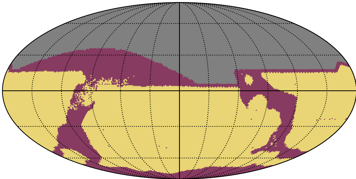
weather_cloudso12v3.4_10yrs All sky: RapidRevisits
