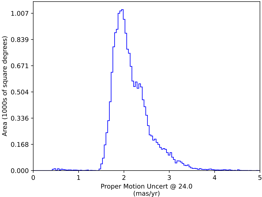
weather_cloudso12v3.4_10yrs WFD: Proper Motion Uncert @ 24.0
