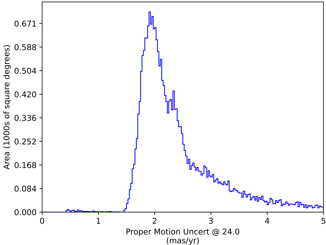
weather_cloudso12v3.4_10yrs All sky: Proper Motion Uncert @ 24.0
