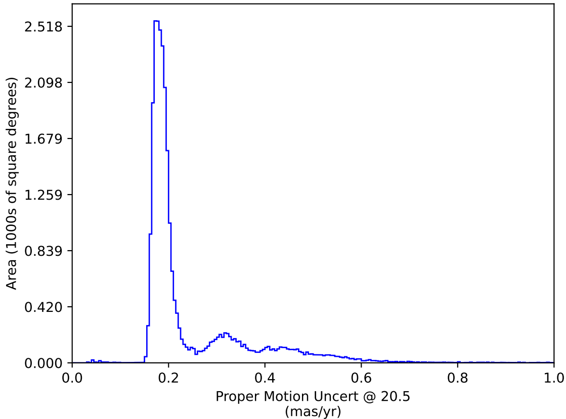
weather_cloudso12v3.4_10yrs All sky: Proper Motion Uncert @ 20.5
