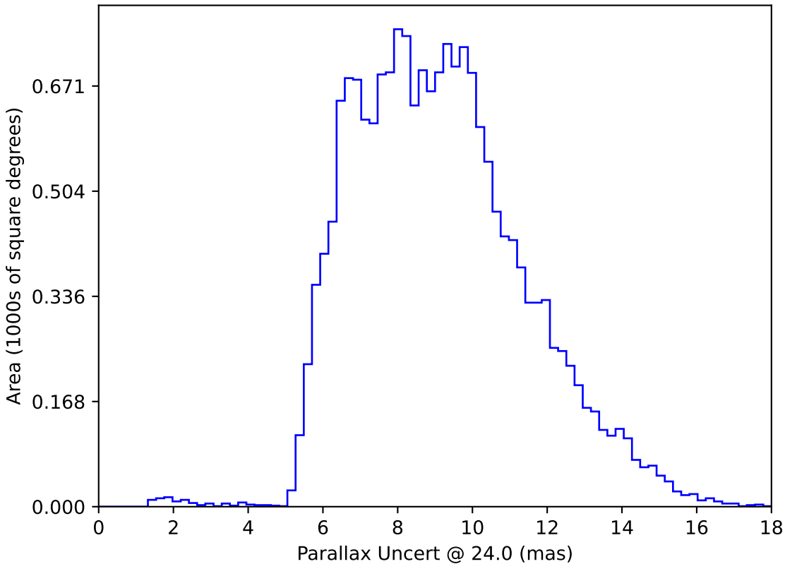
weather_cloudso12v3.4_10yrs WFD: Parallax Uncert @ 24.0
