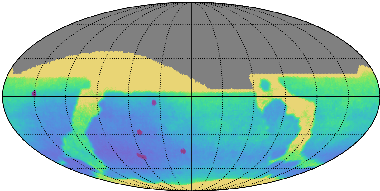
weather_cloudso12v3.4_10yrs All sky: Parallax Uncert @ 24.0
