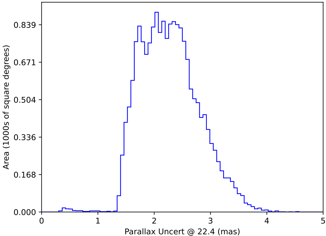
weather_cloudso12v3.4_10yrs WFD: Parallax Uncert @ 22.4
