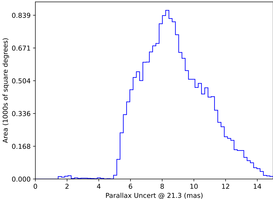
weather_cloudso12v3.4_10yrs WFD y band only: Parallax Uncert @ 21.3
