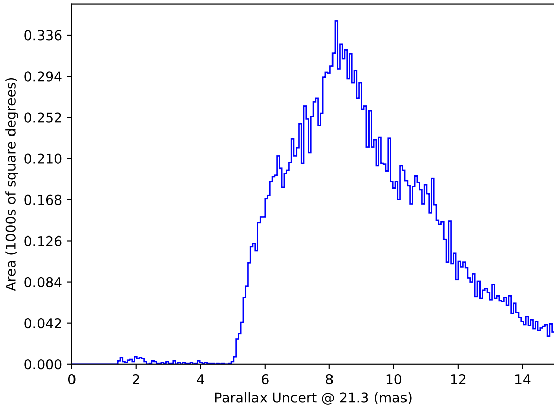
weather_cloudso12v3.4_10yrs All sky y band only: Parallax Uncert @ 21.3
