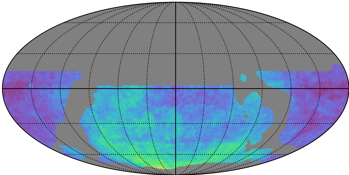
weather_cloudso12v3.4_10yrs WFD: Parallax Coverage @ 24.0
